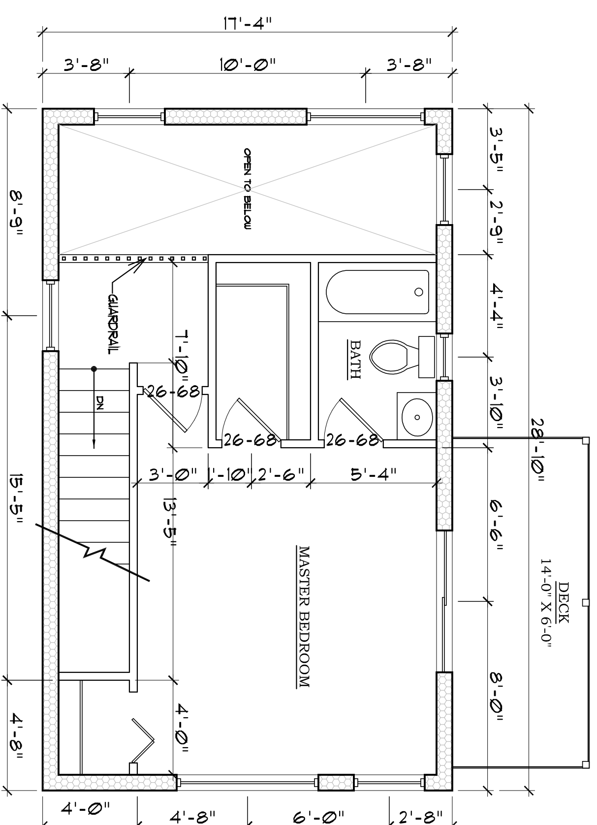
2 2nd Floor North Plan SCALE: 1/4" = 1'-0" 461 SF.
