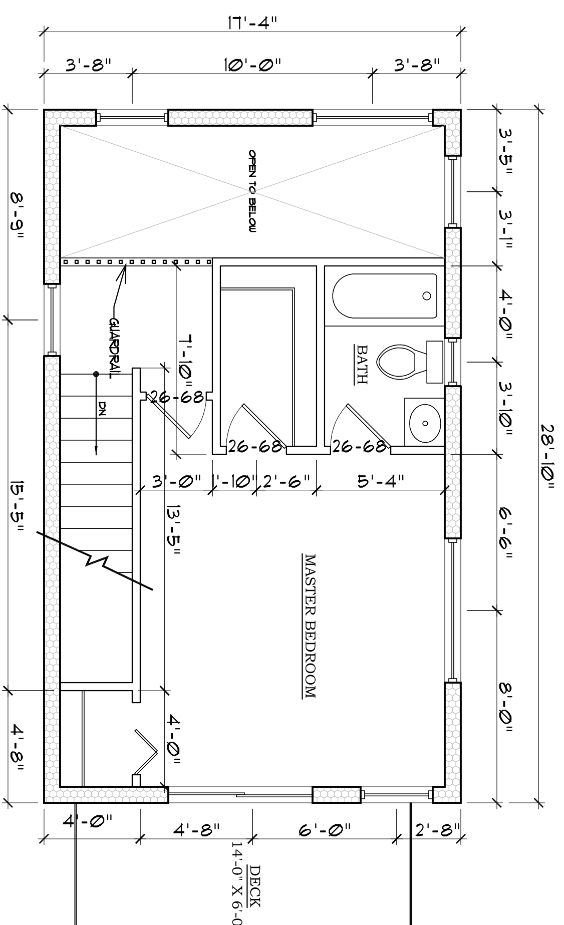
2 2nd Floor North Plan SCALE: 1/4" = 1'-0" 461 SF.
